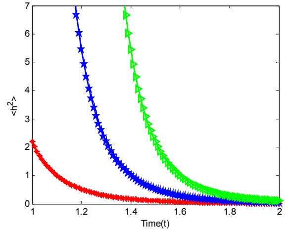
Figure 5. Energy decay curves for A = 7.791 \times 10^{-4} and B = -0.170 , t_0 = 0.4, 0.7, \text{ and } 0.9 .
