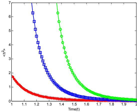
Figure 2. Energy decay curves for A = 1.971 \times 10^{-4} and B = -0.144 , t_0 = 0.4, 0.7, \text{ and } 0.9 .
