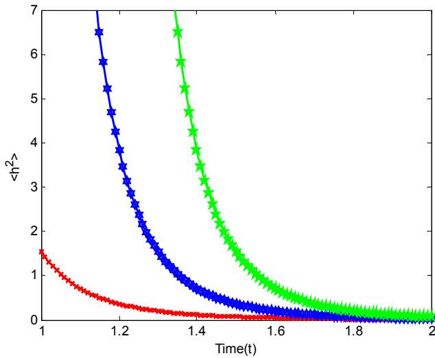
Figure 8. Energy decay curves for A = 1.577 \times 10^{-3} and B = -0.120 , t_0 = 0.4, 0.7, \text{ and } 0.9 .
