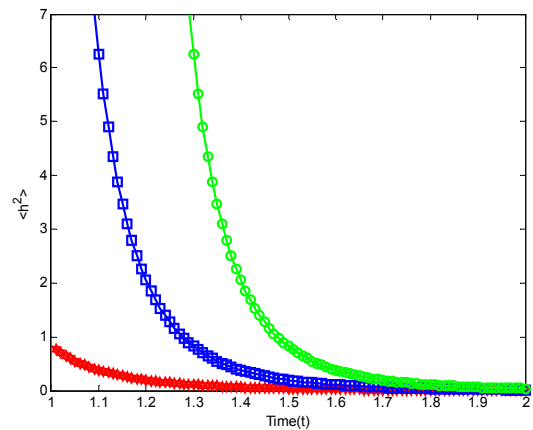
Figure 1. Energy decay curves for A = 6.97 \times 10^{-5} and B = 0.064 , t_0 = 0.4, 0.7, \text{ and } 0.9 .
